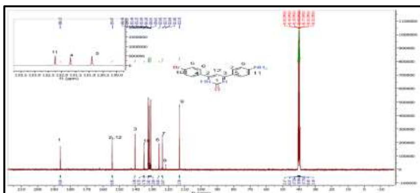
Fig. 4. 13 C-NMR spectrum of compound (A)
