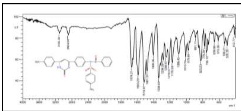
Fig. 11. IR spectrum of compound (B1)
