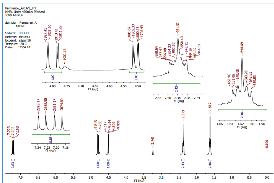
Fig. 2. ^1\text{H} -NMR spectrum of divinyl adipate.
