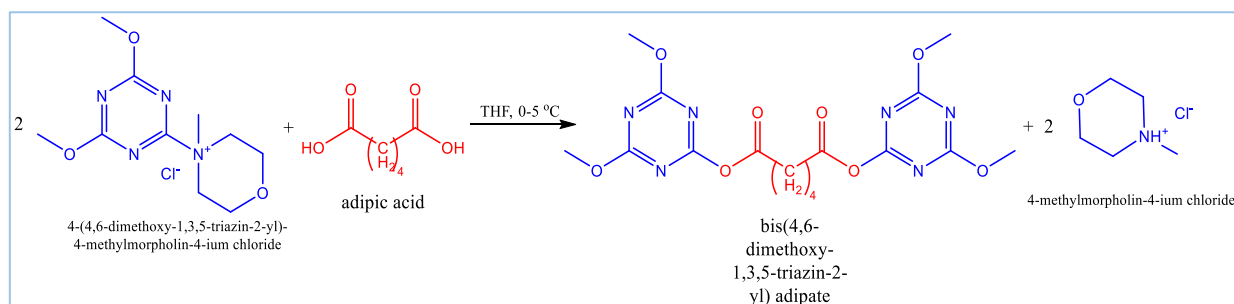
Scheme 4
