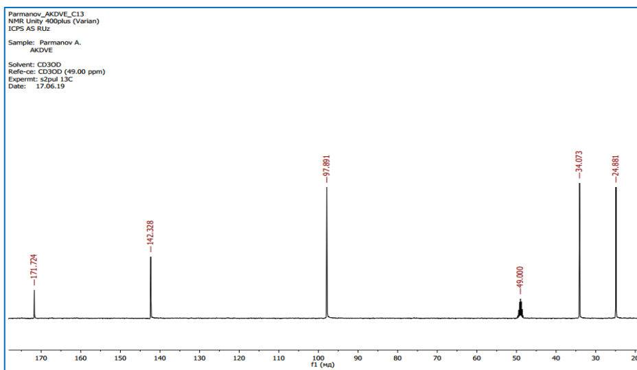
Fig. 3. ^{13}\text{C} -NMR spectrum of divinyl adipate.
