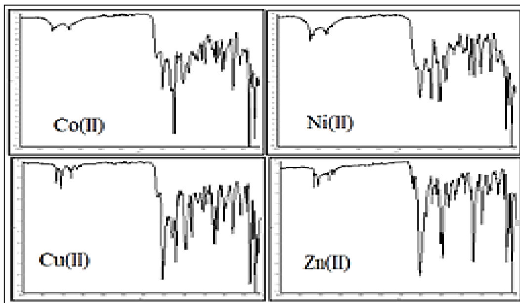
Fig. 4. FT-IR spectra of mixed ligand complexes [MeL(phe)(H 2 O) 2 ]
