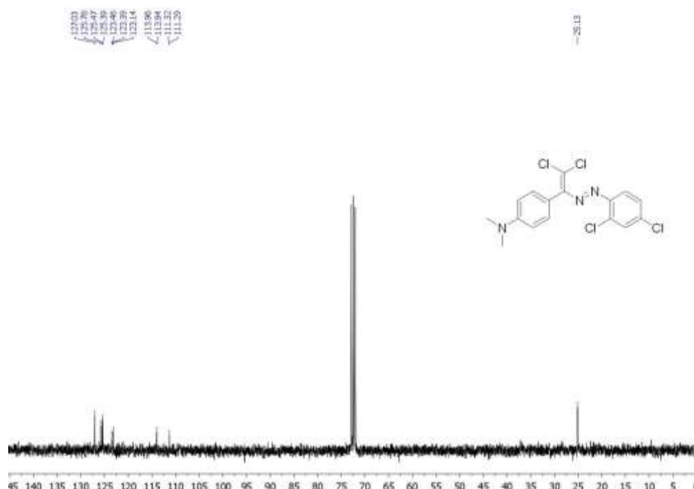
Fig. 2. ^{13}C NMR spectrum of synthesized compound in CDCl_3 solution.
