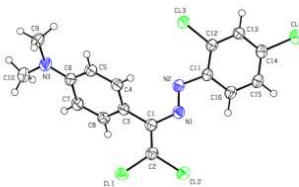
Fig. 3. The molecular structure of the title compound, showing the atom labelling and displacement ellipsoids drawn at the 50% probability level.
