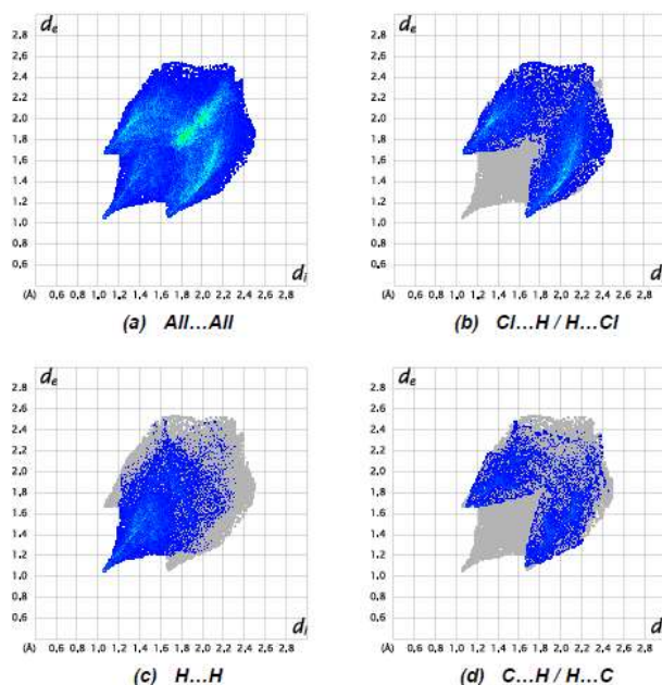
Fig. 8. The full two-dimensional fingerprint plots for the title compound, showing (a) all interactions, and delineated into (b) \text{Cl}\cdots\text{H}/\text{H}\cdots\text{Cl} , (c) \text{H}\cdots\text{H} and (d) \text{C}\cdots\text{H}/\text{H}\cdots\text{C} interactions. The d_i and d_e values are the closest internal and external distances (in Å) from given points on the Hirshfeld surface.
