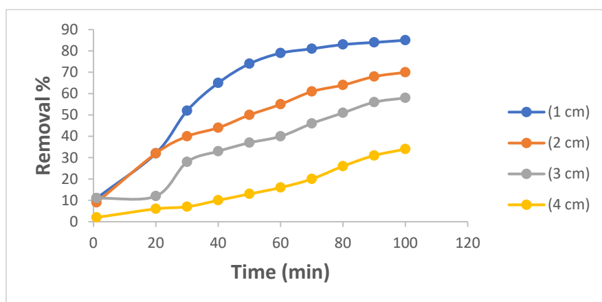
Fig. 5. A graph of the effect of changing the distance between the electrodes on the dye removal rate
