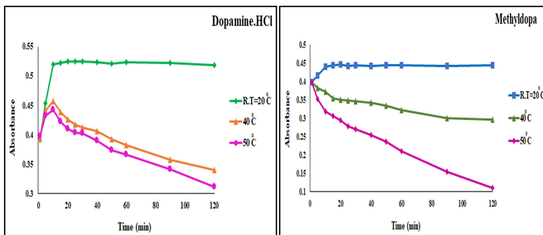
Fig. 7. Effect of temperature and stability time
