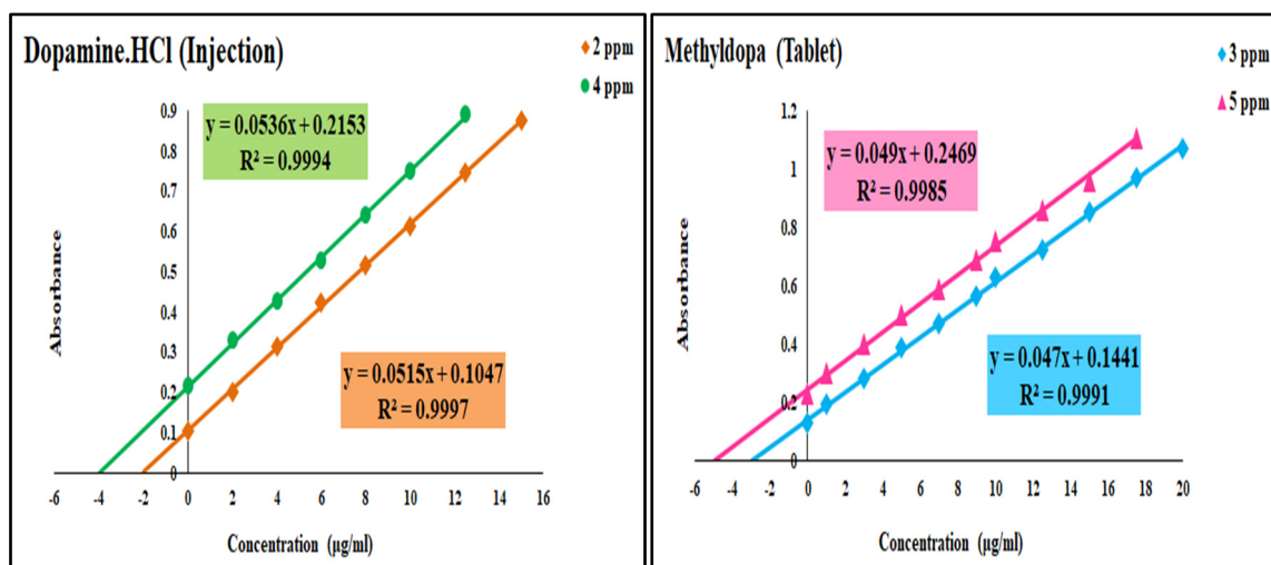
Fig. 13. The standard addition to the pharmaceutical preparation
