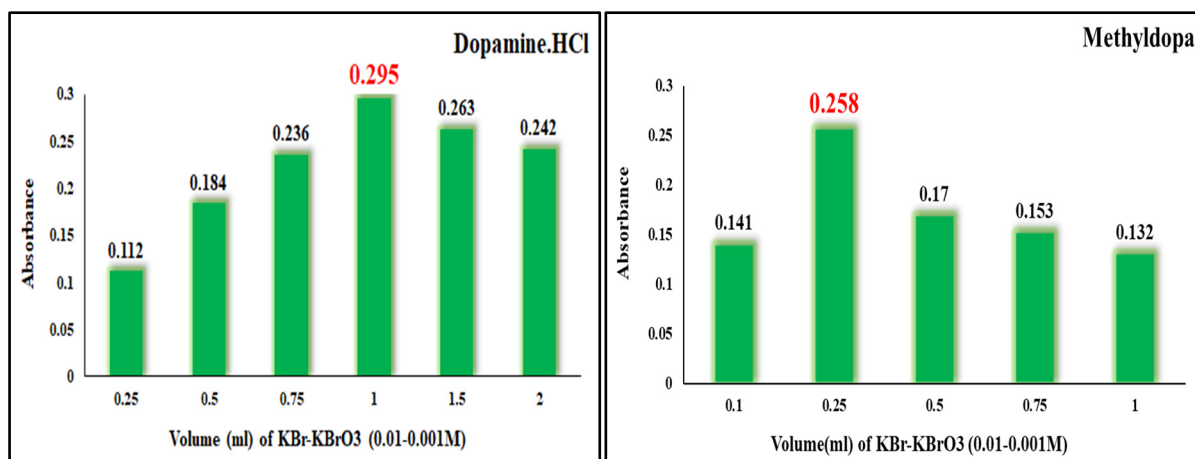
Fig. 2. Effect of increasing amounts of KBr-KBrO 3
