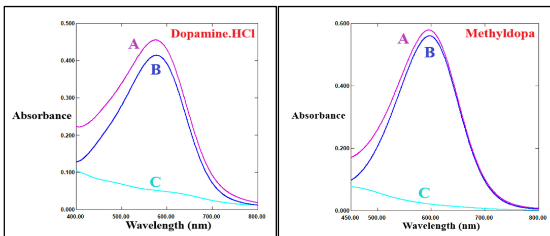
Fig. 8. Final absorption spectrum of dopamine hydrochloride and methyldopa. (A) Absorption spectra of dopamine hydrochloride (8 \mu\text{g/mL} ) and methyldopa (12.5 \mu\text{g/mL} ) versus distilled water. (B) Absorption spectra of dopamine hydrochloride (8 \mu\text{g/mL} ) and methyldopa (12.5 \mu\text{g/mL} ) versus their blank solution. (C) Absorption spectra of their blank solution versus distilled water
