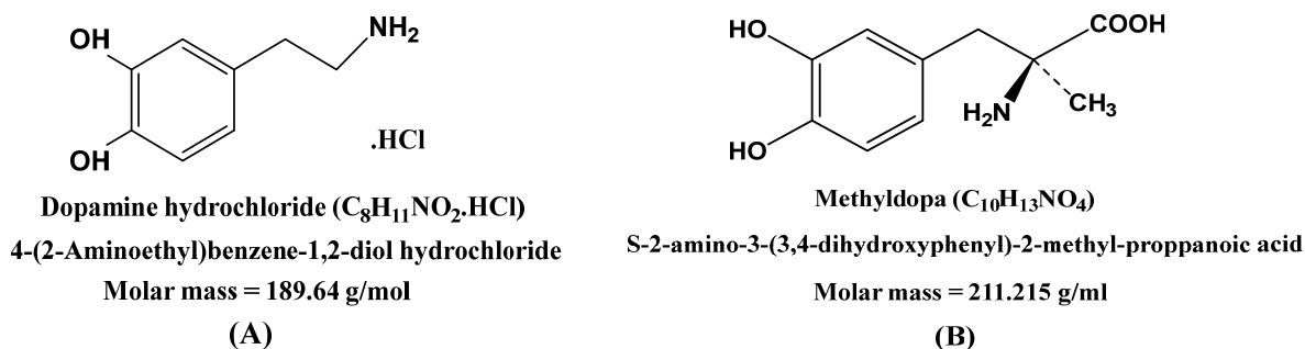
Fig. 1. Chemical formula of dopamine hydrochloride and methyl dopa
