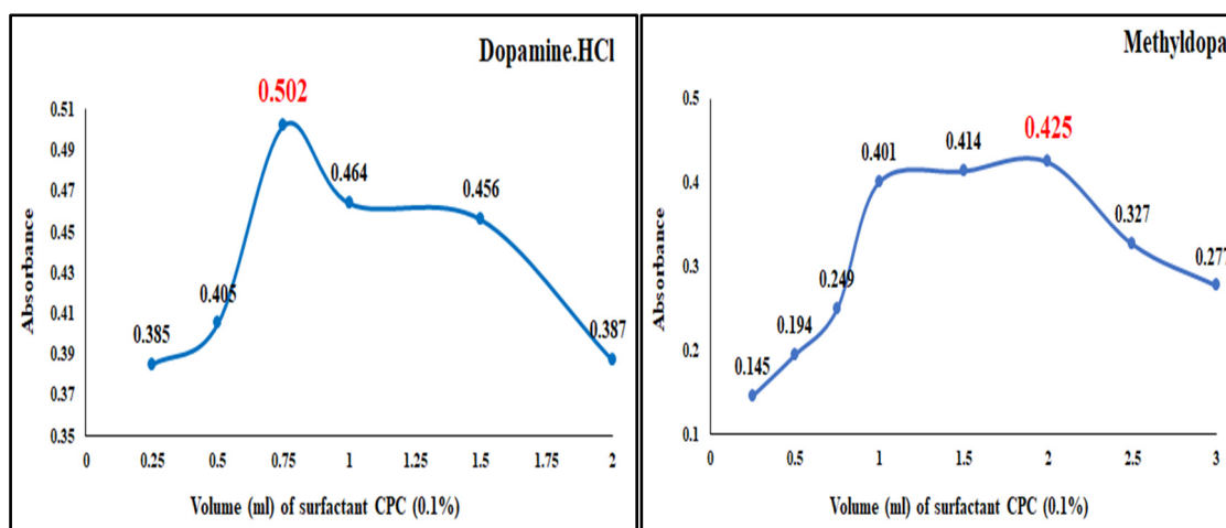
Fig. 6. Effect of increasing amounts of CPC surfactant
