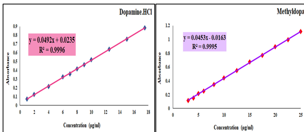
Fig. 9. Standard curves for the drug compounds
