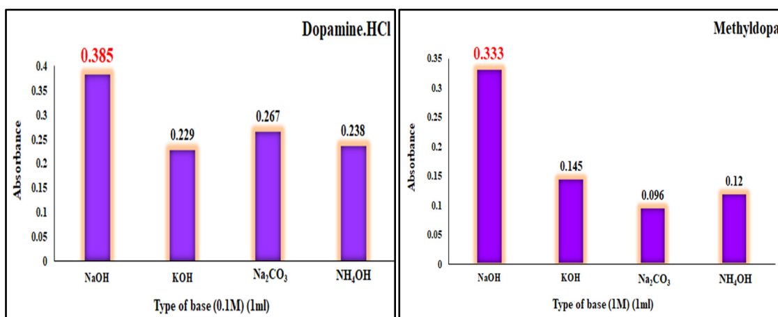
Fig. 4. Effect of different types of bases
