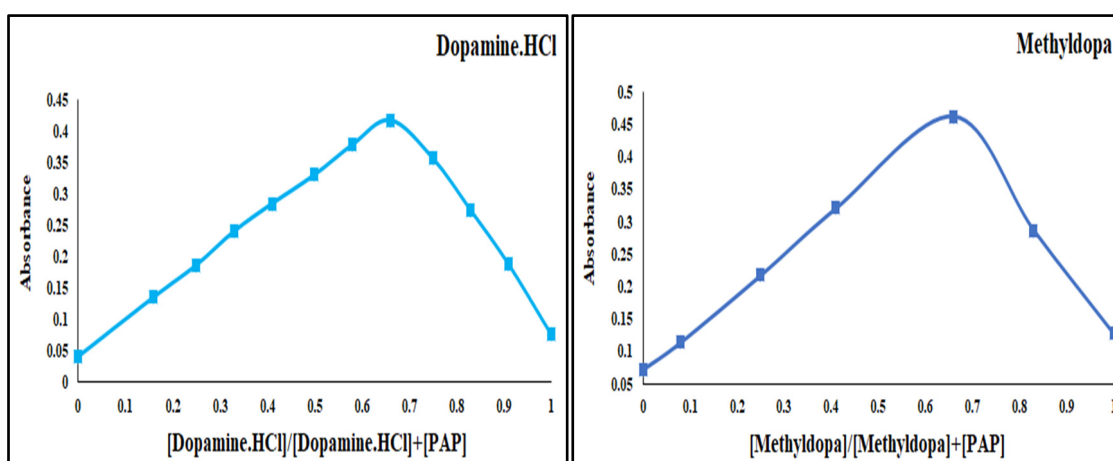
Fig. 10. Continuous changes for dopamine hydrochloride and methyldopa
