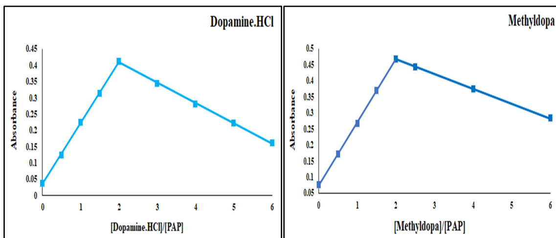
Fig. 11. Molar ratio of dopamine hydrochloride and methyldopa
