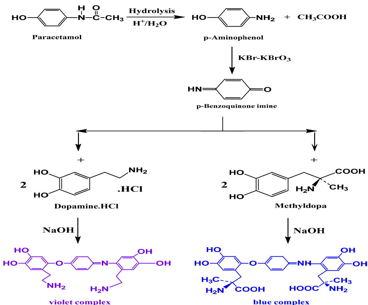
Fig. 12. Suggested interaction mechanism of dopamine hydrochloride and methyldopa
