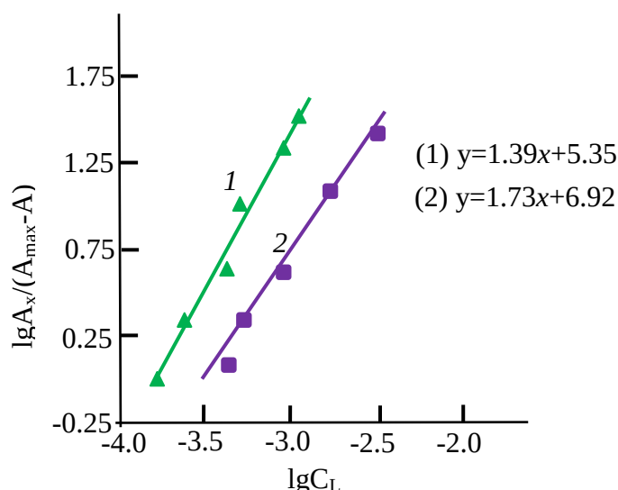
Fig.2. Determination of the HTP-to-Ni (straight line 1) and the An-to-Ni (straight line 2) molar ratios by the mobile equilibrium method. C_{Ni} = 3.4 \times 10^{-5} M , C_L = 1.2 \times 10^{-3} M , C_{An} = 2.0 \times 10^{-3} M , \lambda = 550 \text{ nm} , KFK-2, \ell = 0.5 \text{ cm} .
