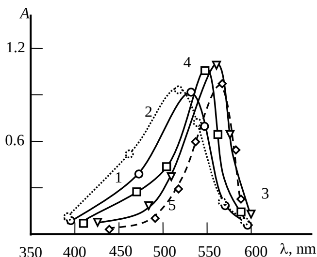
Fig. 1. Absorption spectra of nickel complexes with L and An.
