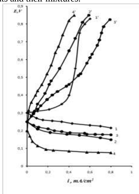
Fig. 1. Cathode, anode polarization curves of St. 3 in a 3% NaCl solution with the addition of an inhibitor, mg/1: 1–1' - without inhibitor; 2–2'–NaNO 2 -100; 3–3'–MEA – 100; 4–4'– NaNO 2 –100 + MEA – 100
