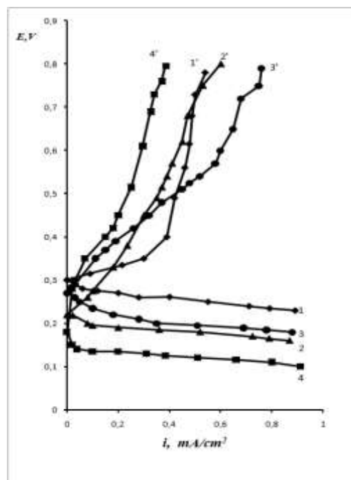
Fig. 2. Cathode and anode polarization curves of St. 3 in a 3% NaCl solution with the addition of an inhibitor, mg/l: 1–1'- without inhibitor; 2–2'– K_2CrO_4 10; 3–3' – H_2N - CH_2 - CH_2 - OH - 90 ; 4–4'– K_2CrO_4 - 10 + H_2N - CH_2 - CH_2 - OH - 90
