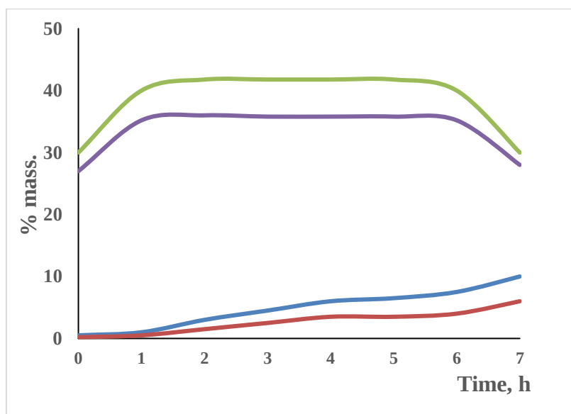
Fig. 2. Dependence of the yield of ΣC 5 -C 6 fraction and the accumulation of coking products on the operating time of the catalysts 5%W/KH-4/Al 2 O 3 and 5%Zn/KH-4/Al 2 O 3
