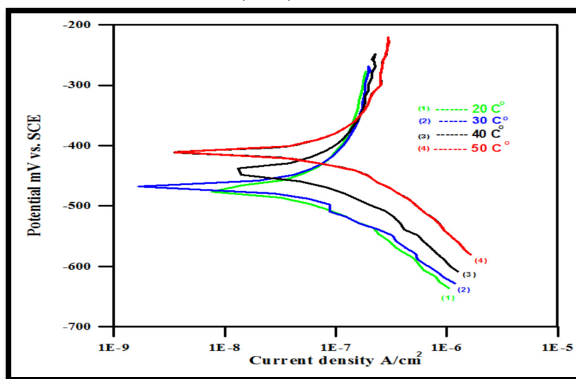
Fig. 5. Tafel plots of CS in chloride containing simulated concrete solution (2.5% NaCl) at 293, 303, 313, and 323 K
