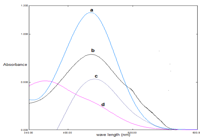
Fig. 7. Final absorption spectrum. (A) absorption spectrum of the dye with acid vs. blank; (B) absorption spectrum of the reaction product vs. water; (C) absorption spectrum of the reaction product vs. blank; (D) blank absorption spectrum vs. water
