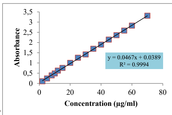
Fig. 2. Standard calibration curve for the dye
