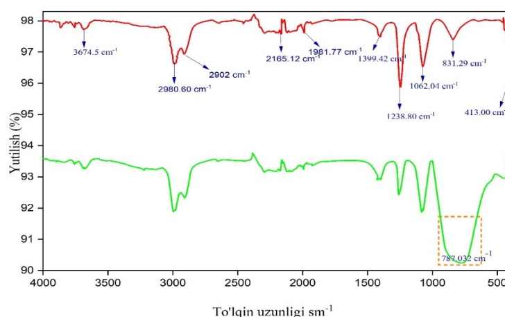
Fig. 8. IR spectrum of titanium dioxide nanotubes \text{TiO}_2 and \text{TiO}_2/\text{PMNS} nanocomposites
