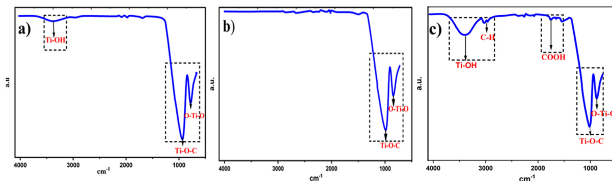
Fig. 2. IR spectrum of titanium dioxide TiO 2 nanotubes obtained after anodization
