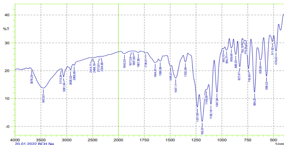
Fig. 4. IR spectrum of 2-sulfonaphthalene
