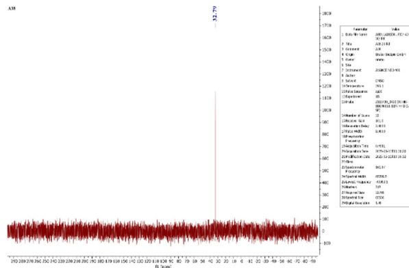
Fig.12. 31 P-NMR spectrum of the compound A 38
