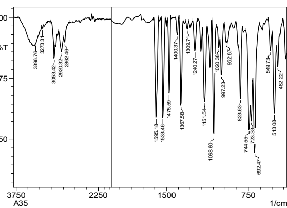
Fig. 8. FT-IR spectrum of compound A 35
