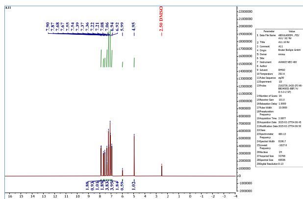
Fig. 3. ^1\text{H} -NMR spectrum of the compound A11.
