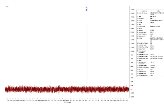
Fig. 14. 31 P-NMR spectrum of the compound A 41
