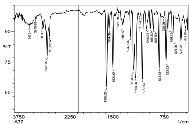
Fig. 7. FT-IR spectrum of compound A 32
