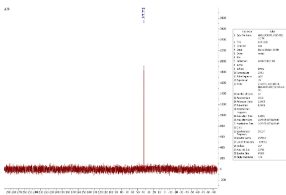
Fig. 13. 31 P-NMR spectrum of the compound A 39 .
