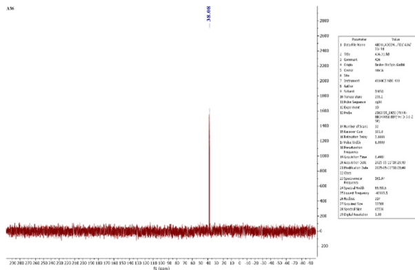
Fig.11. 31 P-NMR spectrum of the compound A 36 .
