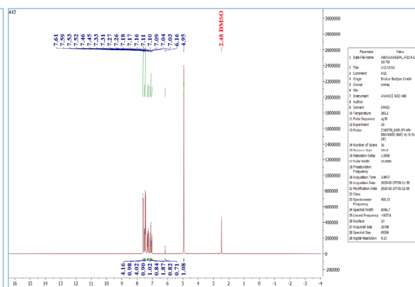
Fig. 4. ^1\text{H} -NMR spectrum of the compound A12
