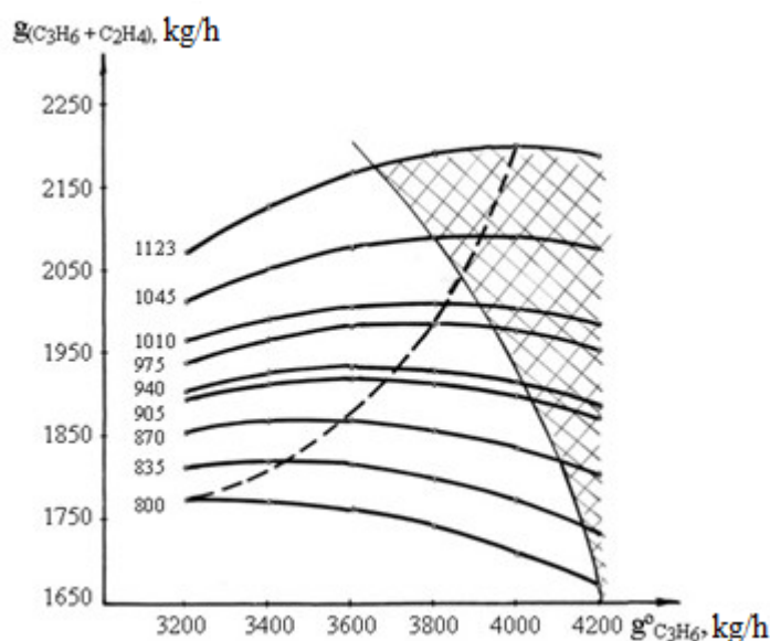
Figure. Determination of optimal inlet temperatures T=(800-1123)^{\circ}K depending on the total reactor load ( g_{C_3H_8}^0=3200-4200 kg/h).
