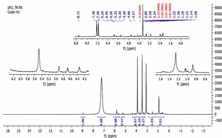
Fig. 4. ^1\text{H-NMR} spectra of compound H1
