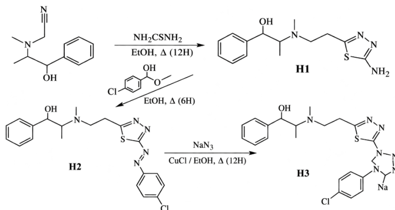
Scheme 1. Synthetic steps for preparation of derivatives[H 1 ],[H 2 ],[H 3 ]
