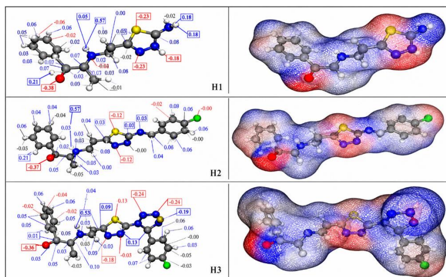
Fig. 10. Atomic Charge for components (H1-H3)
