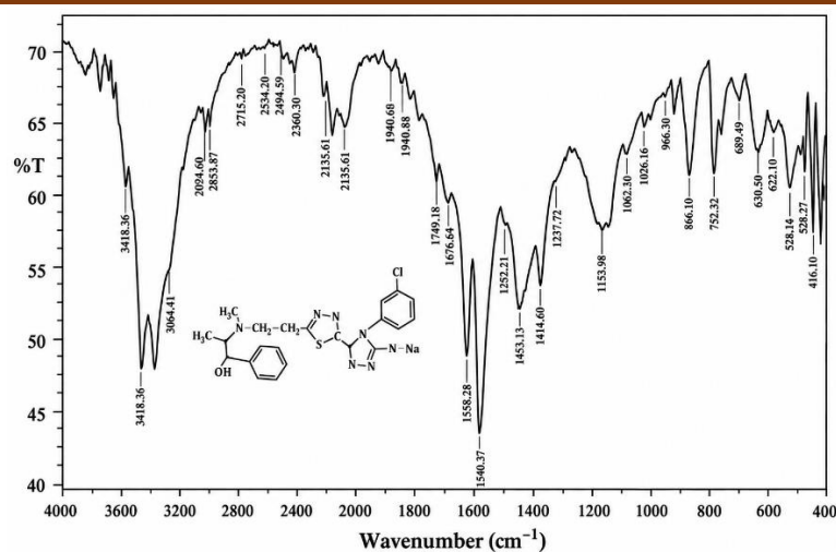
Fig. 3. FTIR spectrum of compound H3
