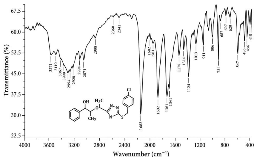
Fig. 2. FTIR spectrum of compound H2
