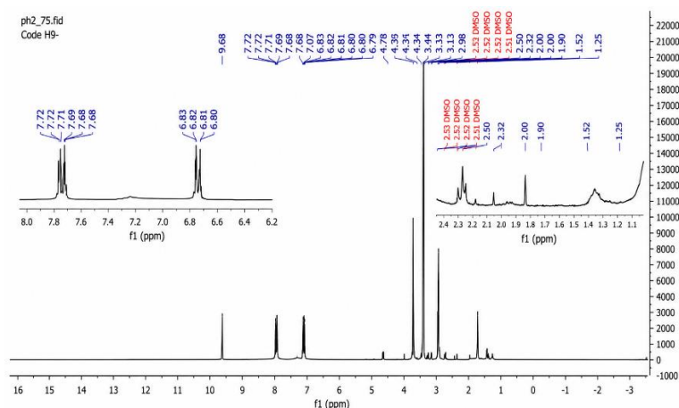
Fig. 5. ^1\text{H-NMR} spectra of compound H2
