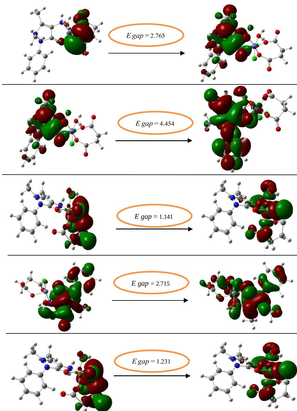
Fig. 4. HOMO and LUMO orbitals of the synthesized metal complexes (1-5)
