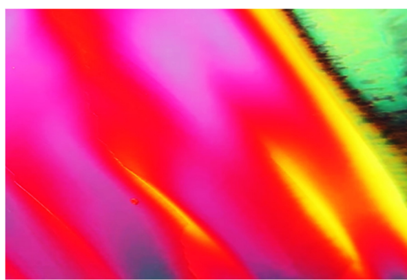
Fig. 10. The nematic phase of [E5] during heating
