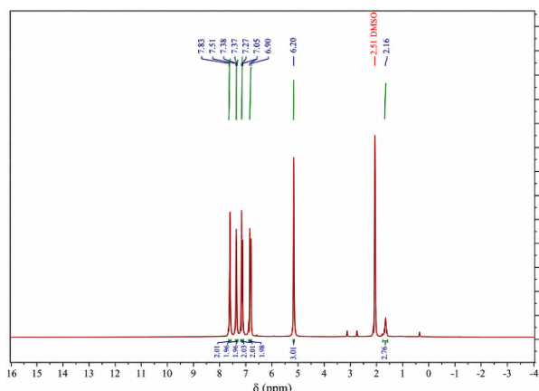
Fig 3. ^1\text{H} -NMR spectrum of the compound \text{E}_6
