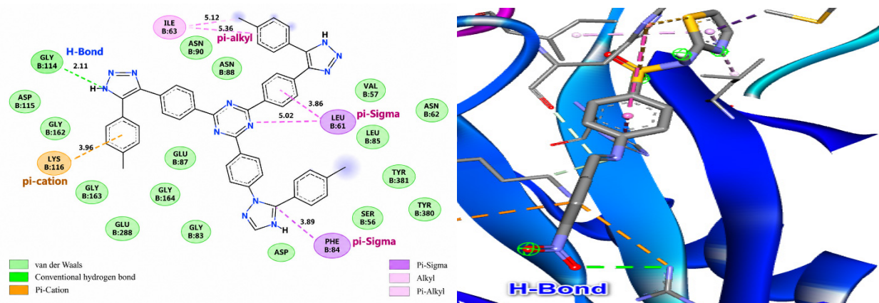
Fig. 8. 3D and 2D dimensions of compound [E8]
