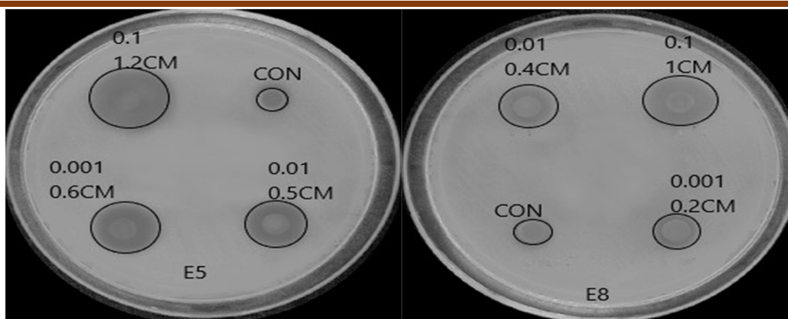
Fig. 6. The inhibition of compounds E5 and E8 against Staph. aureus .
