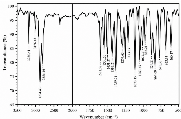
Fig 2. FT-IR spectrum for the compound E 8
