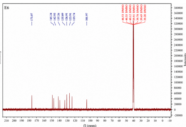
Fig 4. ^{13}\text{C} -NMR spectrum of the compound \text{E}_6
