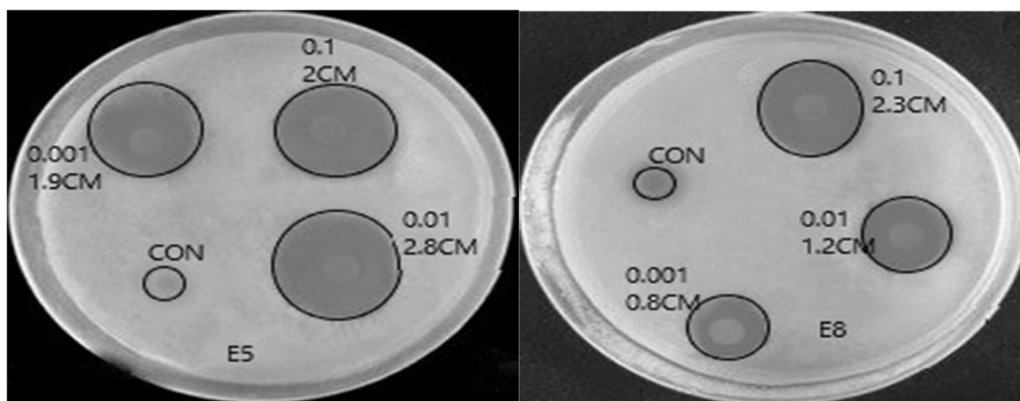
Fig. 5. The inhibition of compounds E5 and E8 against E. coli .
