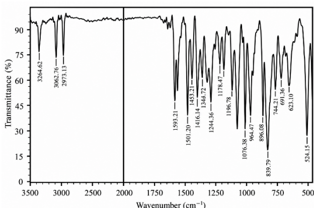
Fig 1. FT-IR spectrum for the compound E 6
